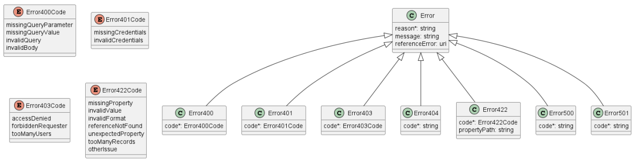
Figure 9. Data model types to represent an erroneous response
